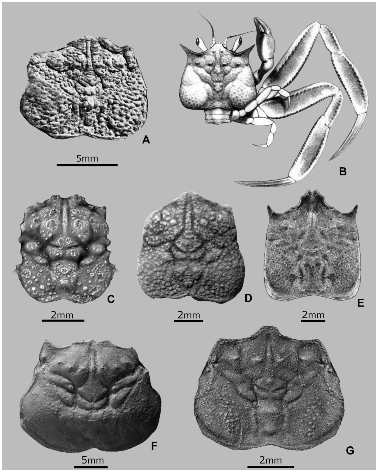
Fig. 6. Telamonocarcinid crabs (Eubrachyura, Dorippoidea) known to date. A, B. Telamonocarcinus gambalatus Larghi, 2004, from Cenomanian–Turonian strata in central-western Lebanon, Hgula and Haqil: A. holotype (MSNMi26033; see Larghi, 2004, fig. 4). B. reconstruction of appearance in life (see Larghi, 2004, fig. 5). C. Navarrara betsieae Klompmaker, 2013, from upper Albian Aldoirar patch reef (Albeniz Unit, Eguino Formation) of Koskobilo, northern Spain: compilation photograph based on MGSB77705 and MAB k.3004 (see Klompmaker, 2013, fig. 4g). D. Personadorippe kalashnikovi gen. et sp. nov., holotype (MWO 1 9298), from the lower Cenomanian (Lyaminsk Formation, Schloenbachia varians ammonite Zone), Moscow Oblast, Dmitrovsky district, village of Nikolskoye. E. Withersella crepitans Wright and Collins, 1972 (NHMUK IC15; see Schweitzer and Feldmann, 2011, fig. 7) from the Aptian, Isle of Wight, United Kingdom. F. Eodorippe spedeni Glaessner, 1980, holotype (NZGSAR 675; see Luque, 2014a, fig. 2e), Campanian–Maastrichtian, New Zealand, Te Hoc River. G. Telamonocarcinus antiquus Luque, 2014a, 2014b, holotype (IGM p881012; see Luque, 2014a, fig. 2a) from lower Albian (Tablazo Formation) of Colombia, department of Santander, near the town of La Fuente.
