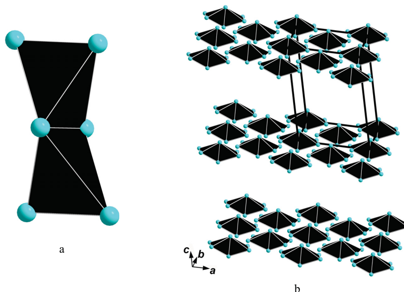
Fig. 9. The [\text{O}_2\text{Cu}_6] dimer of the oxocentred tetrahedra \text{OCu}_4 (a) and the motif formed by these dimers in the structure of cryptochalcite/cesiodymite (b). The unit cell is outlined in (b).
