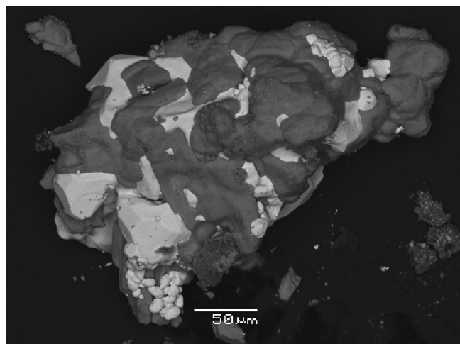
Fig. 3. Crusts of cesiodymite overgrowing anglesite crystal cluster. SEM picture in secondary electrons (anglesite is white, cesiodymite is grey).
