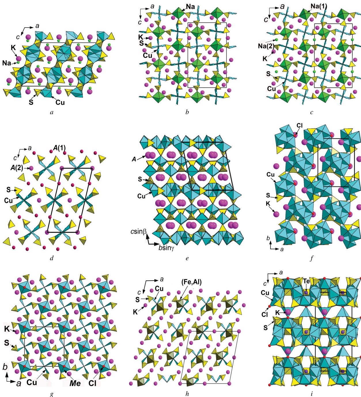
Fig. 10. Crystal structures of euchlorine ( a : drawn after Scordari & Stasi, 1990), wulfite ( b ) and parawulfite ( c ) (both drawn after Pekov et al. , 2014a), eleomelanite ( d : drawn after Pekov et al. , 2016), cryptochalcite/cesiodymite ( e , this work), kamchatkite ( f : drawn after Varaksina et al. , 1990), piypite ( g : drawn after Effenberger & Zemmann, 1984), klyuchevskite ( h : drawn after Gorskaya et al. , 1992) and nabokoite ( i : drawn after Pertlik & Zemmann, 1988). The unit cells are outlined. Cu-centred polyhedra for wulfite, parawulfite, eleomelanite, piypite and klyuchevskite are shown as almost flat squares for better clarity; in eleomelanite A(1) = (K, Pb, Ca) and A(2) = (K, Rb, Cs) ; in cryptochalcite/cesiodymite for the content of the A sites see Table 6; the Me site in piypite can be occupied by K, Na and/or Cu^{2+} .
