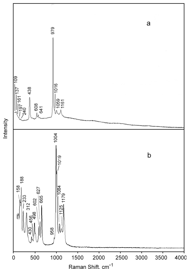
Fig. 5. Raman spectra of cryptochalcite (a) and cesiodymite (b).
