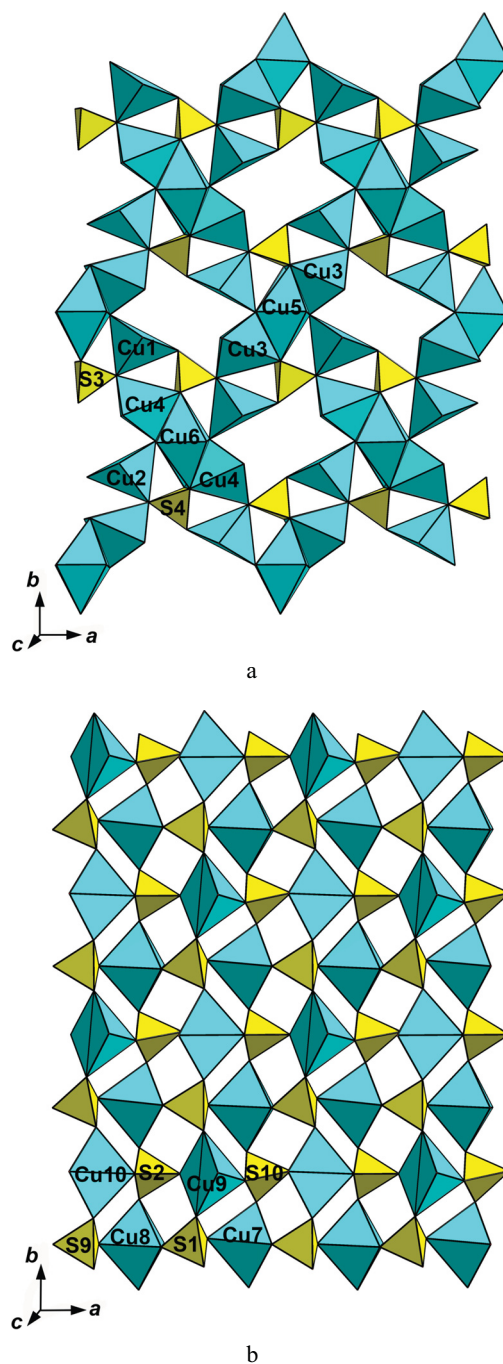
Fig. 8. The layer I (a) and the layer II (b) in the structure of cryptochalcite/cesiodymite projected onto the ab plane.
